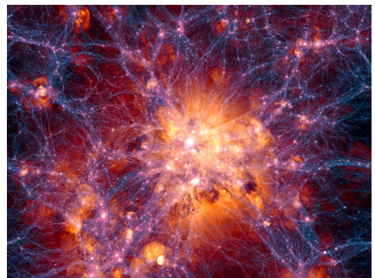
Fig. 16 - The Cosmic Web was evident to the astronomers who observed the cores' motions and recognized the threads that bind them all.
