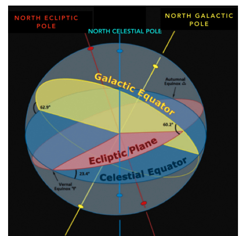
Fig. 6 - The ecliptic, celestial, and galactic Equators form angles that changed long ago, and altered human perceptions.
