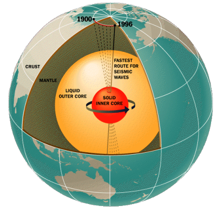
Fig. 12 - The Earth's Solid Inner Core - primary Author of the geomagnetic field - spins faster than the surface.
