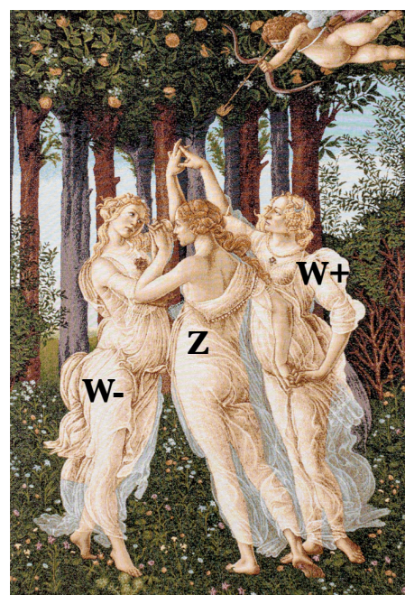
Fig. 11 - The EW Force also interacts with antibodies, which can heal our bodies.
