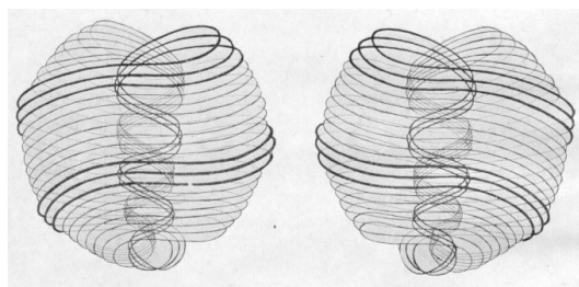
Fig. 9 - These are the "last atoms", drawn by A. Besant and C. Leadbeater, authors of the book "Occult Chemistry", published in 1908.
