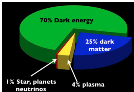
Fig. 4 - Space Sciences can only observe 5% of the total, universal mass they calculate.
