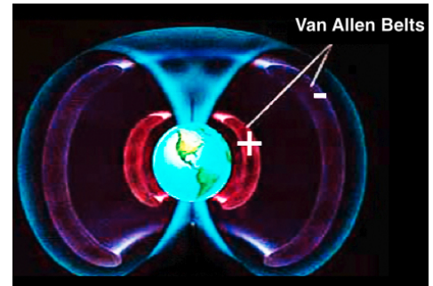
Fig. 3 - An "apple" - Earth's magnetosphere - surrounds the Earth's visible surface and hides the Plasmasphere observed in EUV.
