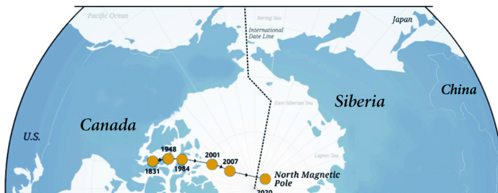
Fig. 2 - The North Magnetic Pole between 1990 and 2005 has accelerated its speed of 0-15 km/year to 50-60 km/year. The intensity of the geomagnetic field is decreasing and going to flip soon. It can be the announced REVELATION.
