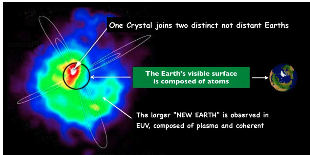
Fig. 1 - A new Earth observed in EUV (left) coexists with the visible Earth (right). The new Earth's coherent oneness indicates the Organic Intelligence in which we, humans, might be partakers if we changed our atomic nuclei state.
