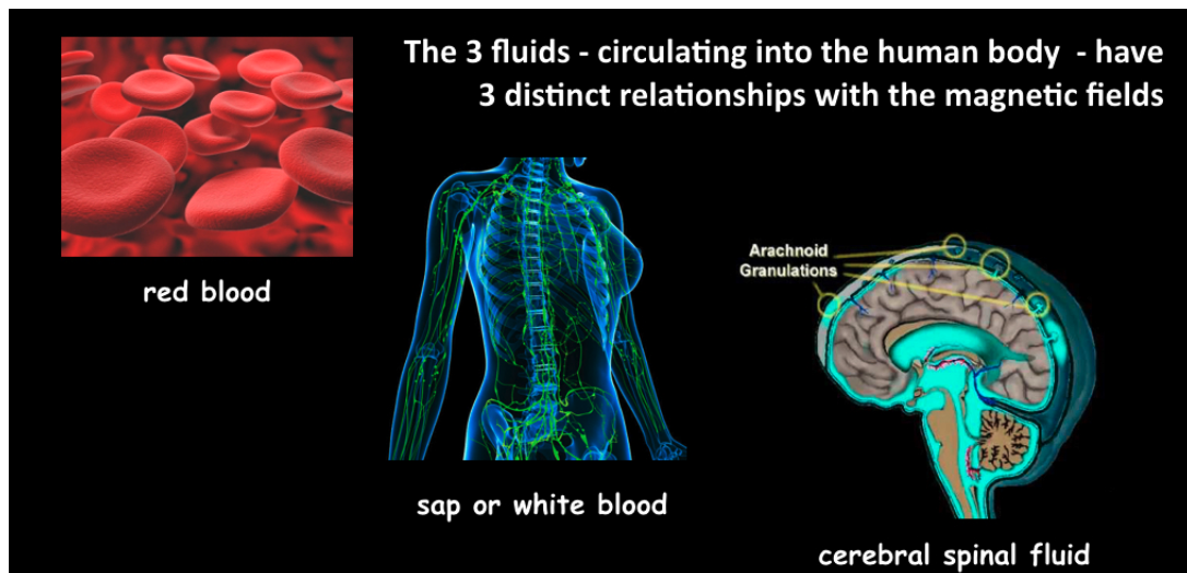
Fig. 5 - Our body's primary fluids - red blood, white blood or lymph, cerebral spinal fluid - interact with five magnetic fields: galactic, solar, interplanetary, first and second geomagnetic fields. All are interacting with each other and quickly changing.
