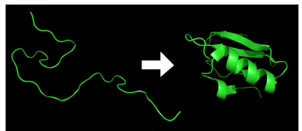
Fig. 14 - Protein folding is a process that enhances the magnetic properties on the electric ones, due to the DNA cooperations with the three tRNA, mRNA, rRNA.
