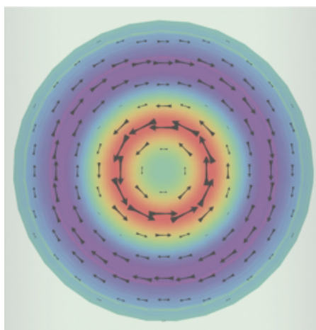
Fig. 8 - The "weak" force exerts an expansive pressure that is much stronger than the confining one created by the "strong" force at its periphery. Are these names appropriate? Not at all. However, a proton is not a brick ; it is the seat of two opposite motions. One is centrifugal hence expansive, stronger than the centripetal , confining one at its periphery. Can we find a new balance between these two forces? We can if we realize their effects on our bodies.
