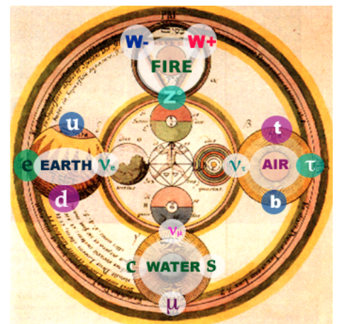
Fig. 20 - This Renaissance picture matches the particles of the Standard Model (Fig. 15), man's eternal firing body.
